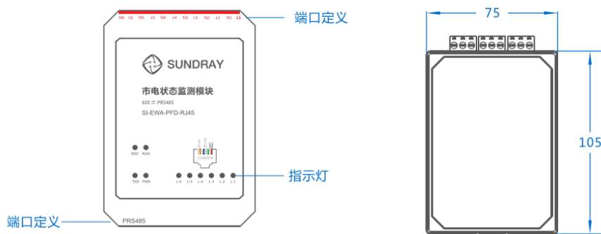
信锐 SI-EWA-PFD-RJ45
